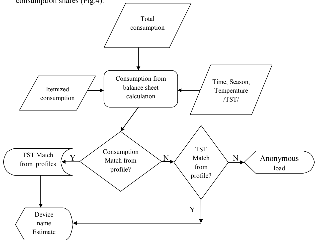
Fig. 6 Estimating permanent load types - basic structure
