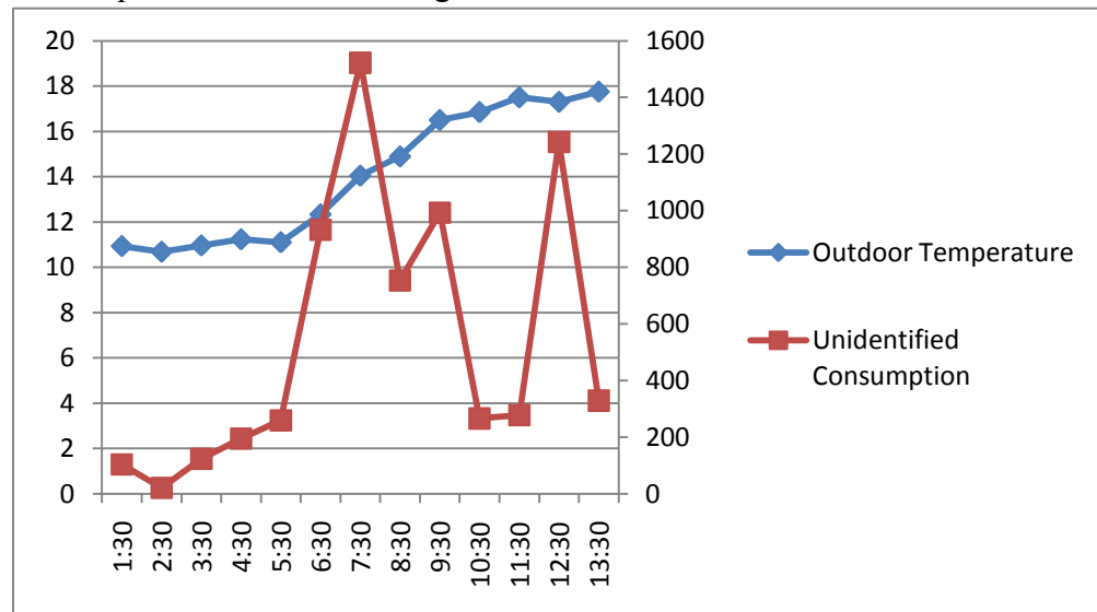
Fig.5 Outdoor temperature and energy consumption of directly connected loads
